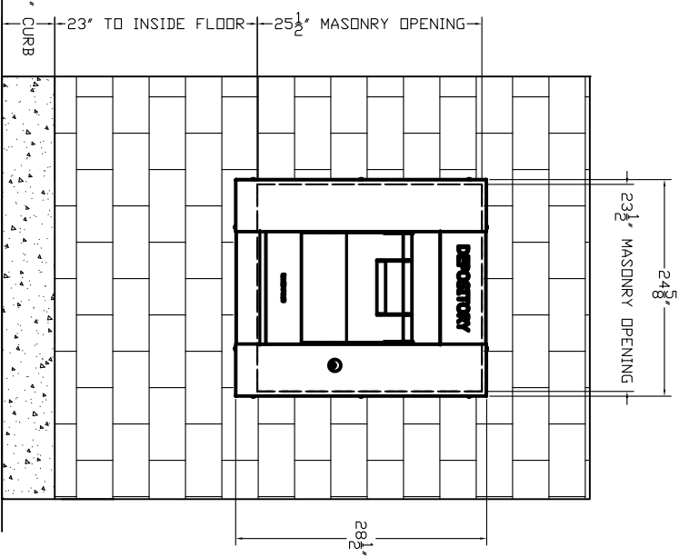
EXTERIOR FLOOR ELEVATION
